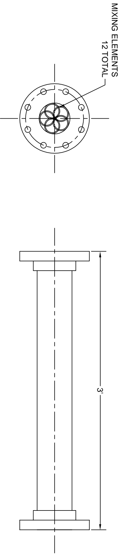
END VIEW
